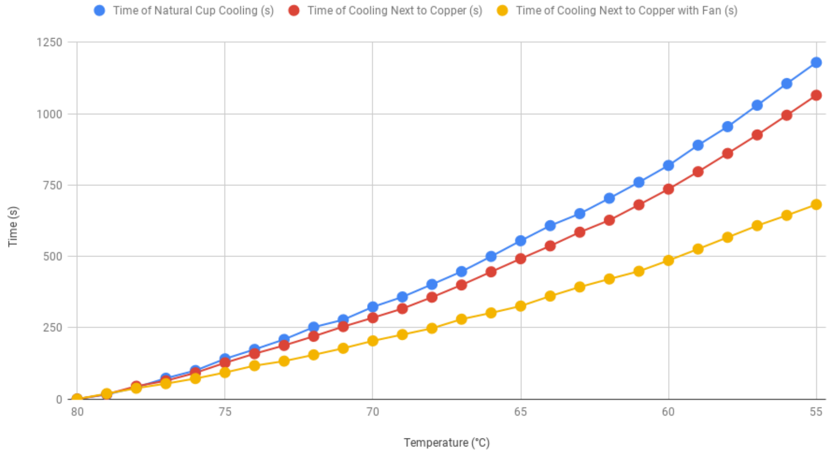
Time of Cup Cooling (s) vs. Temperature (°C)
